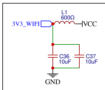
PWR Stabilizer for Slot
